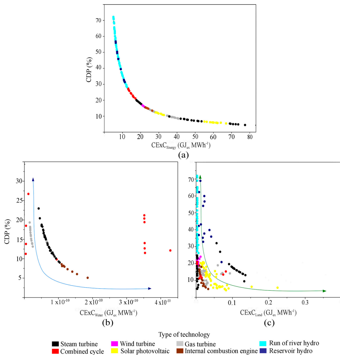
Figure 5. Correlation between CDP and CExC each resources and by type of technology. The specifically CExC for energy resource is depicted in (a); The CExC for water and land resources are shown in (b,c), respectively.
